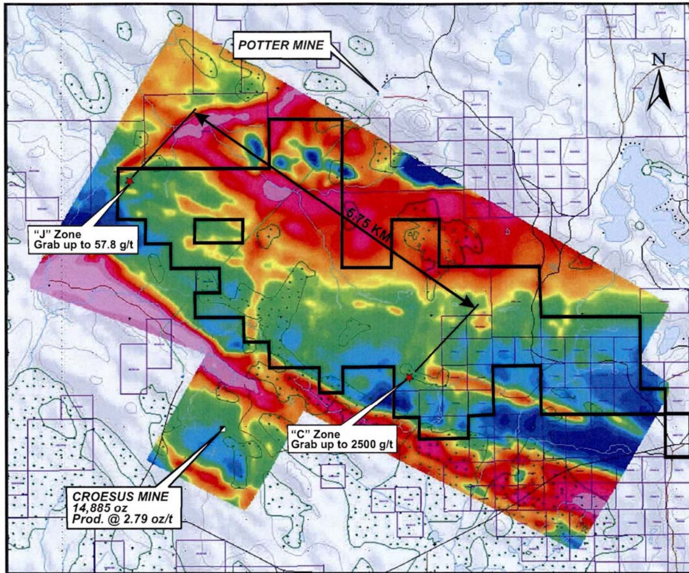
Abitibi Gold Property - Total magnetic survey
